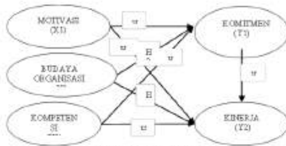
Figure 2. Path Diagram
