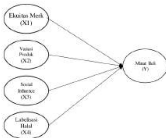
Figure 1. Research Framework
